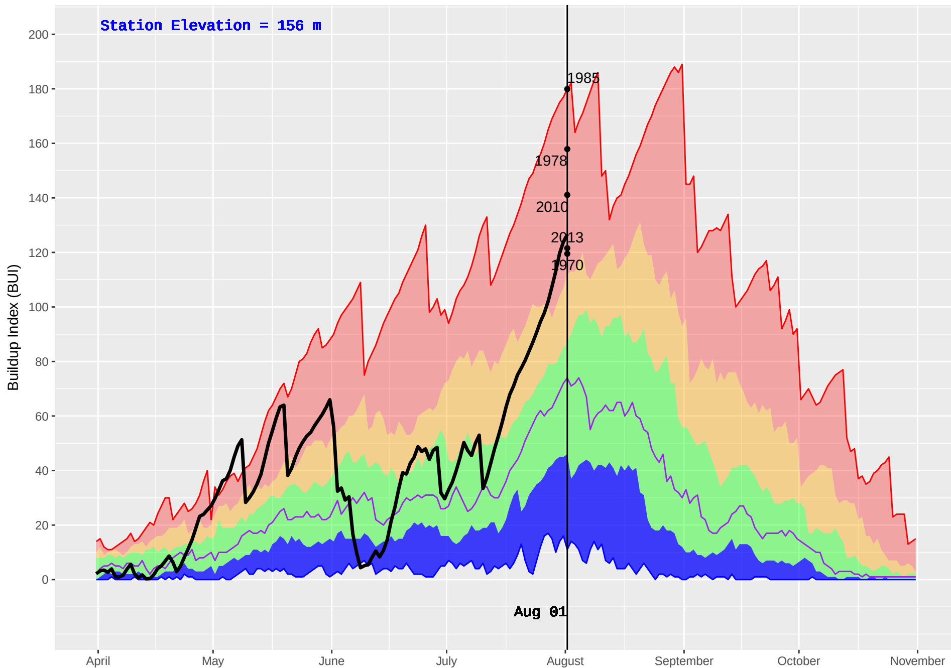
WOSS CAMP (21) : Historical (1970–2016) and Current (2018) Daily Buildup Index (BUI)
