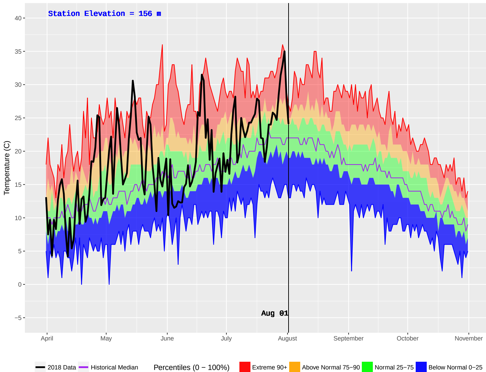
WOSS CAMP (21) : Historical (1970–2016) and Current (2018) Daily Temperature
