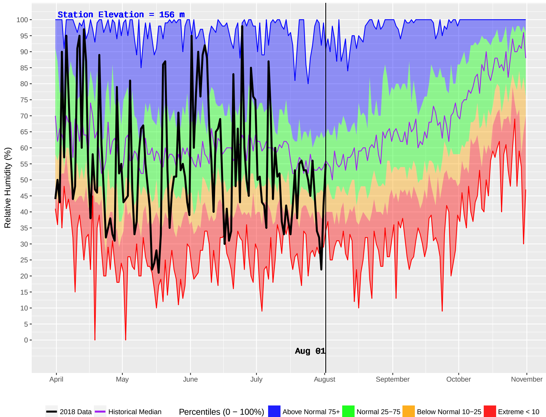
WOSS CAMP (21) : Historical (1970–2016) and Current (2018) Daily Relative Humidity
