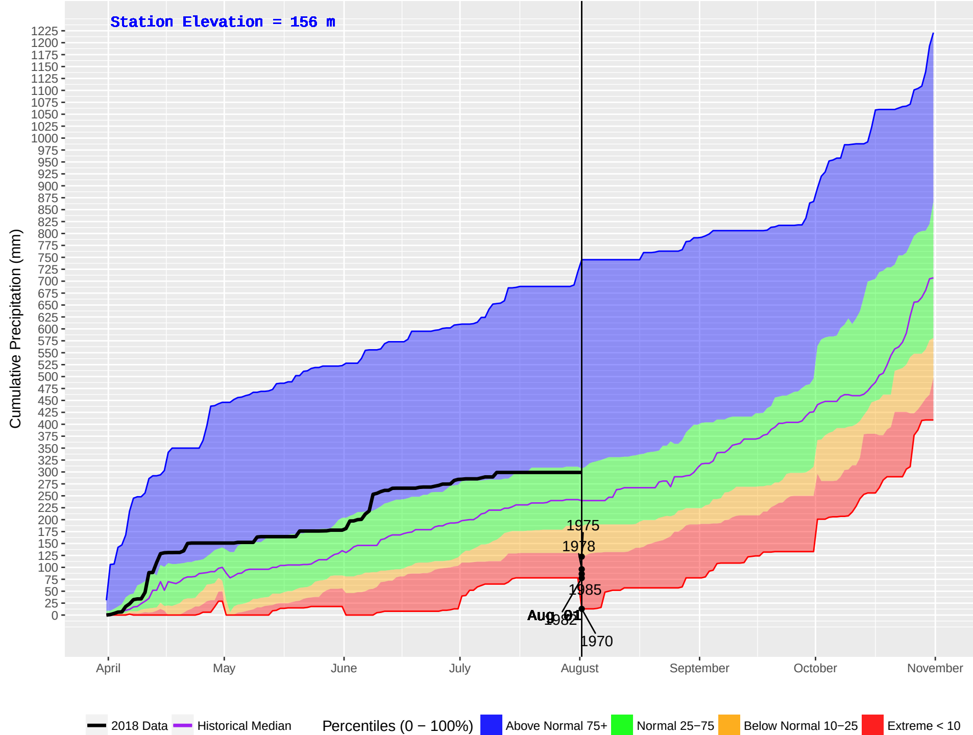
WOSS CAMP (21) : Historical (1970–2016) and Current (2018) Daily Cumulative Precipitation
